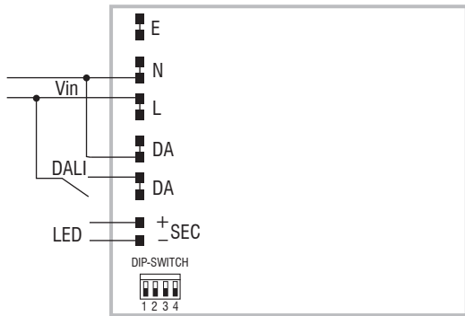
PUSH SWITCH diagram - Collegamento PUSH SWITCH
