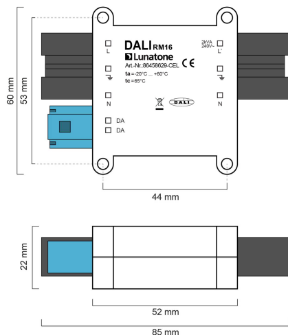
Geometrie RM16-CEL
