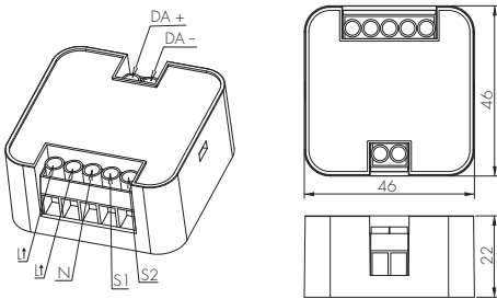
Socket mounting HBTD8200D
