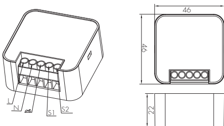
Socket mounting HBTD8200T
