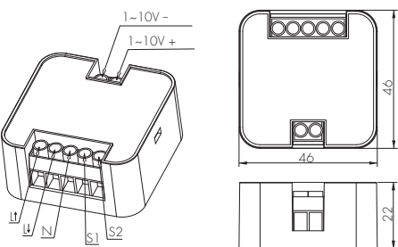
Socket mounting HBTD8200V
