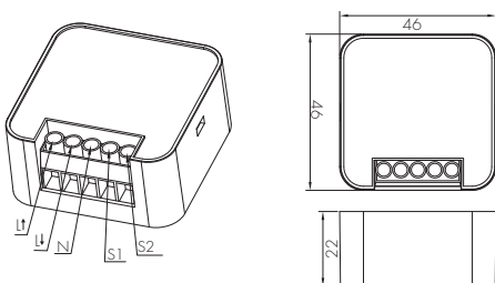
Socket mounting HBTD8200S
