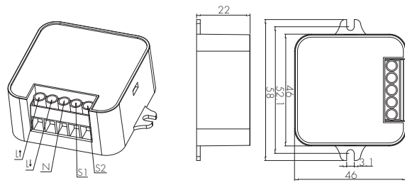
Fixture mounting HBTD8200S/F
