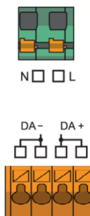
Fig.6. connection plan
