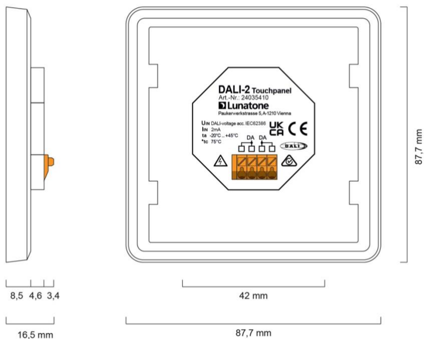
Fig.1. dimensions
