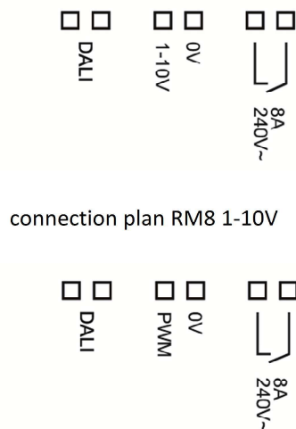
connection plan RM8 PWM
