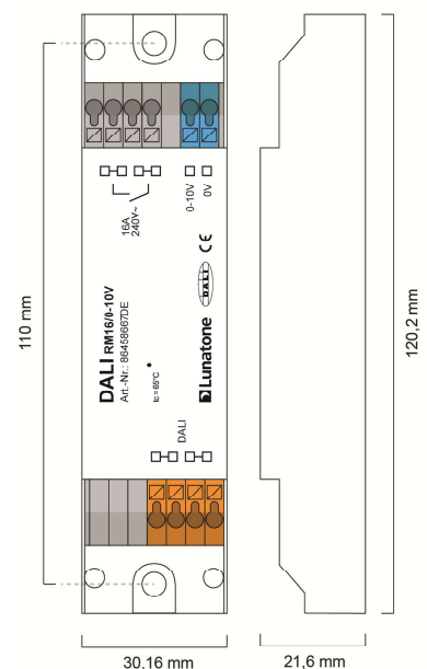
geometry RM16 0-10V DE
