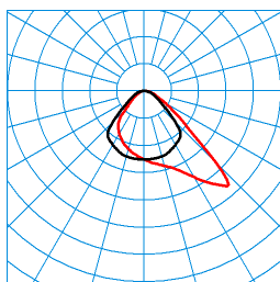
Bicult Act T G2 SMC TGCS 55 ETDI 03 EU (ACTDWW) TX369222 ■ C0 - C180 ■ C90 - C270 DIN 5040: A50 UTE: 1,00 D CEN Flux Code: 59 89 98 100 100 0 0 0 0
