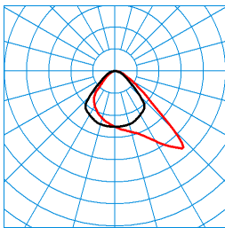
Bicult Act T G2 SMC TGCS 55 ETDI 03 EU (ACTDCW) TX369222 ■ C0 - C180 ■ C90 - C270 DIN 5040: A50 UTE: 1,00 D CEN Flux Code: 59 89 98 100 100 0 0 0 0
