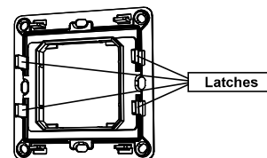
Retaining plate
