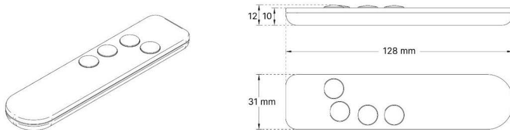
Geometrie wDALI-2 Extra Long Rang Remote
