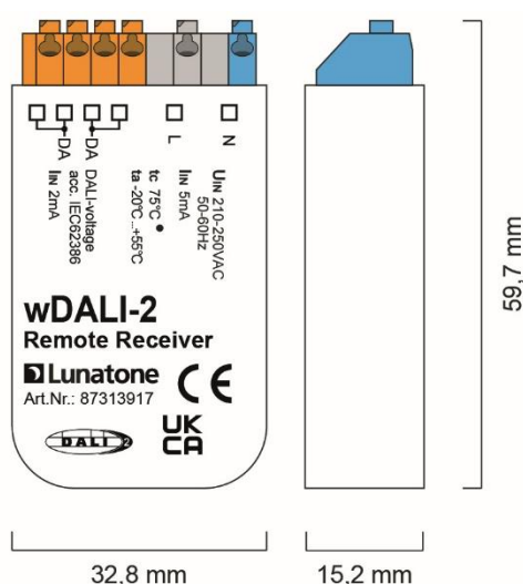
Geometrie wDALI-2 Extra Long Range Receiver, 87313917
