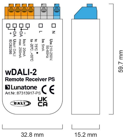
Geometrie wDALI-2 Extra Long Range Receiver PS, 87313917-PS
