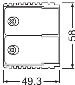
OT CABLE CLAMP B-STYLE
