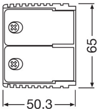
OT CABLE CLAMP A-STYLE
