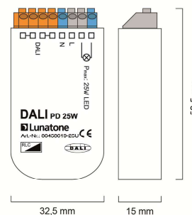
dimension PD
