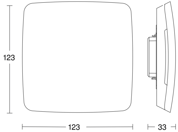
Dimension Drawing
