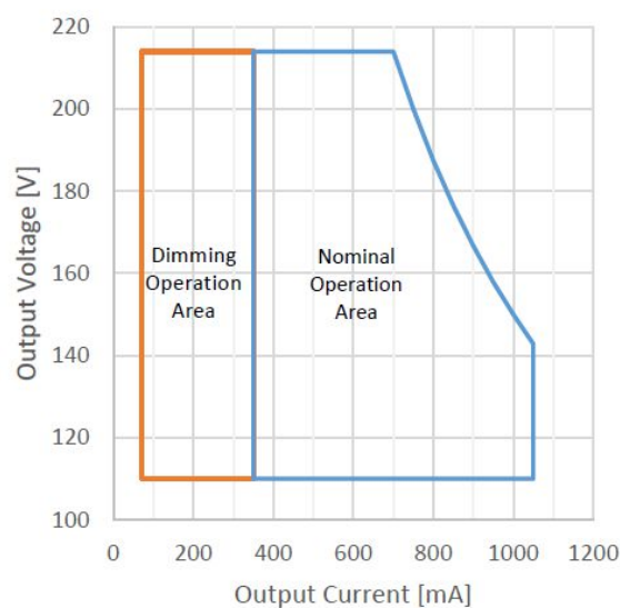
IT DALI 150 120-240 1A0 P7 Operating Window
