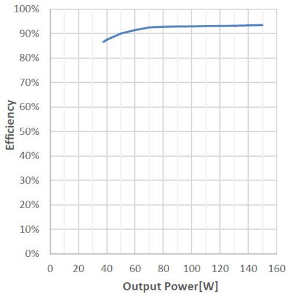
IT DALI 150 120-240 1A0 P7 Typical Efficiency vs. Load
