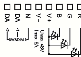
connection plan back box
