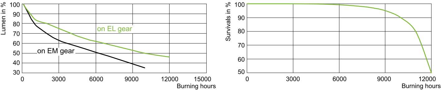
LDLM_CDM-TC_35W_830-Lumen maintenance diagram
