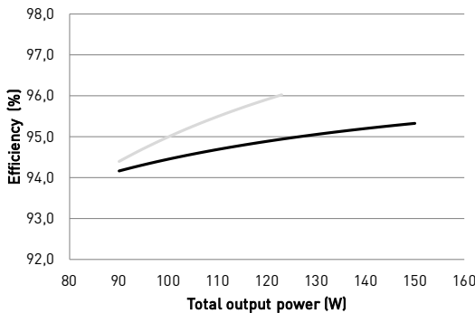
Typical efficiency
