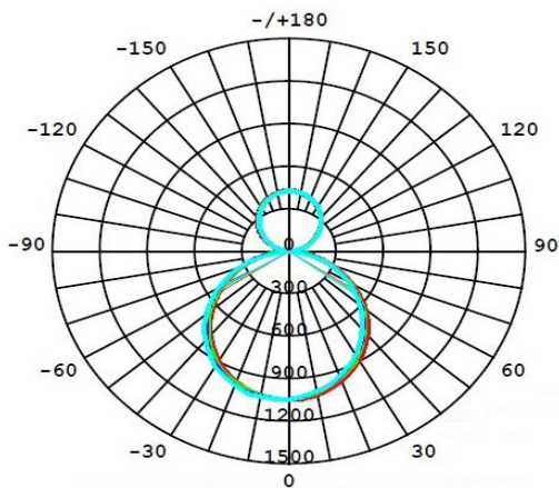
Abb. 3: Abstrahlcharakteristik Up and Down LED Panel 110°
