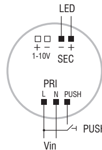
PUSH diagram Collegamento PUSH
