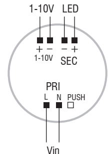
1...10 V diagram Collegamento 1...10 V
