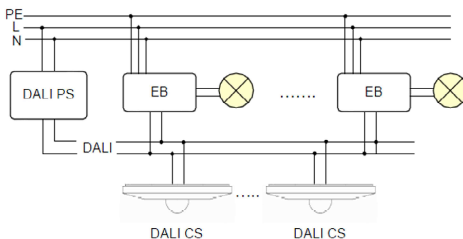
typical installation
