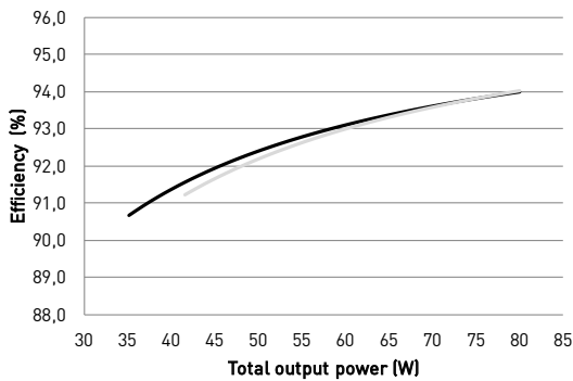
Typical efficiency
