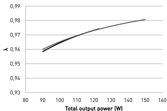
Typical power factor
