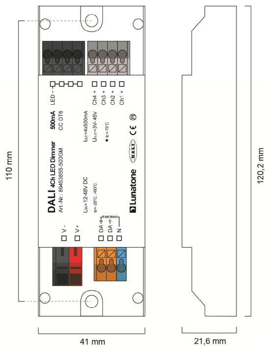
Geometrie GM
