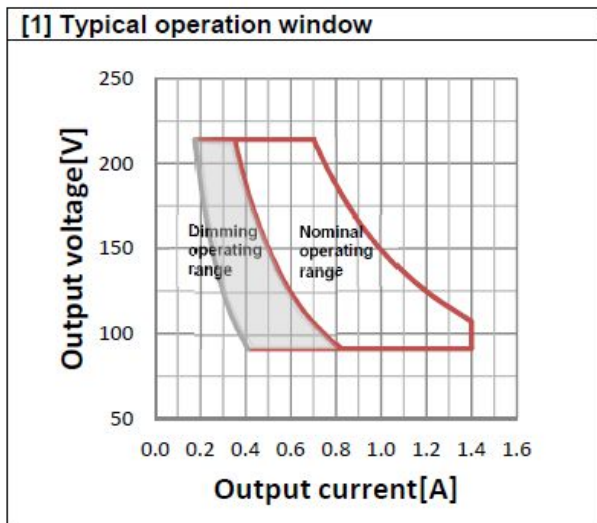
OT 150/220-240/1DIMA 1A4 P7 Operating Window
