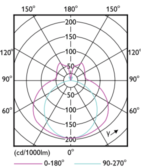
Light Distribution Diagram - CorePro LED PLL HF 12W 840 4P 2G11
