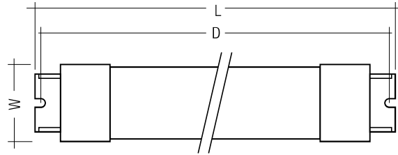
Fig. 1: Stick Connection: blade terminal
