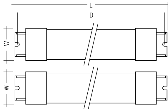
Fig. 2: Stick + Stick Connection: blade terminal
