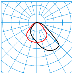
Cultega Act T SMC PAW 600 05 (ACTDSU) TX280853 ■ C0 - C180 ■ C90 - C270 DIN 5040: A40 UTE: 1,00 D CEN Flux Code: 54 85 97 100 100
